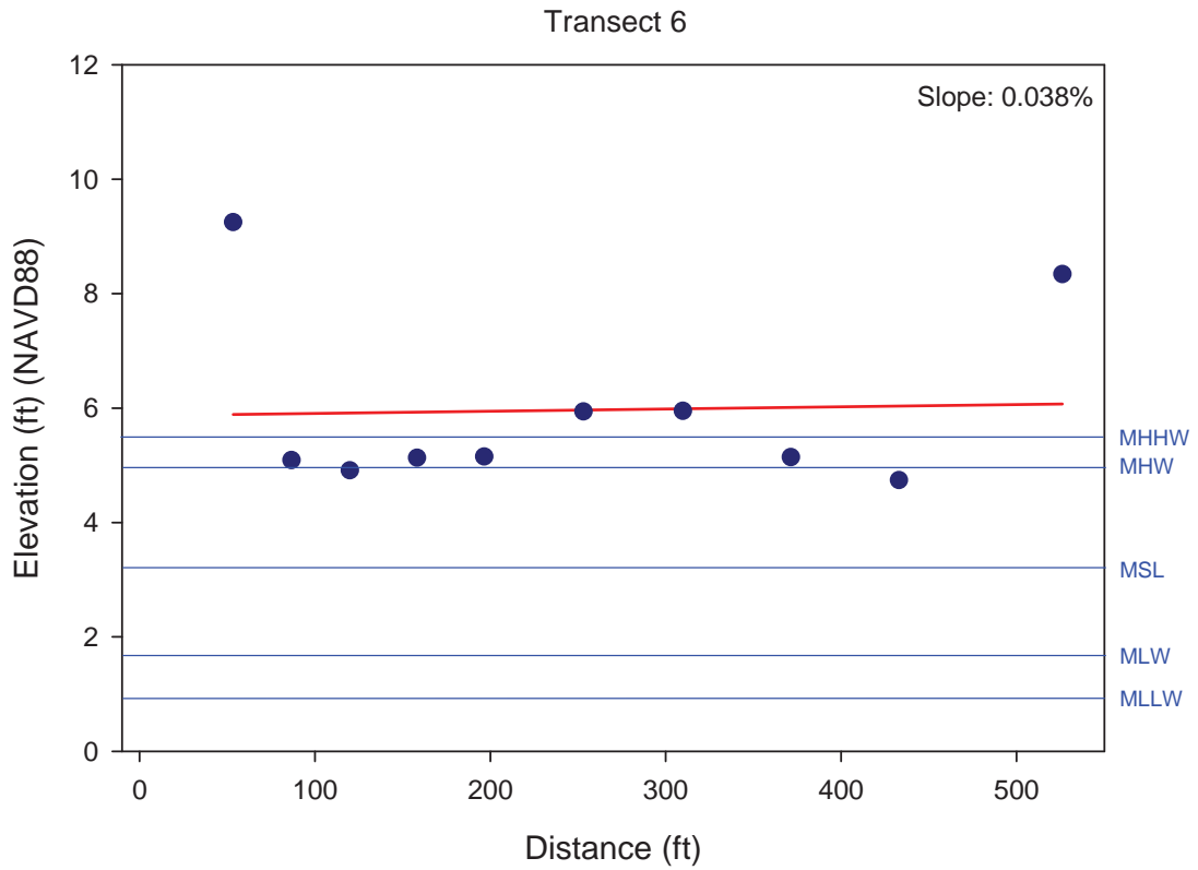
Figure A-7. Transect slopes (elevation vs. distance from 0 ft. to end point).
