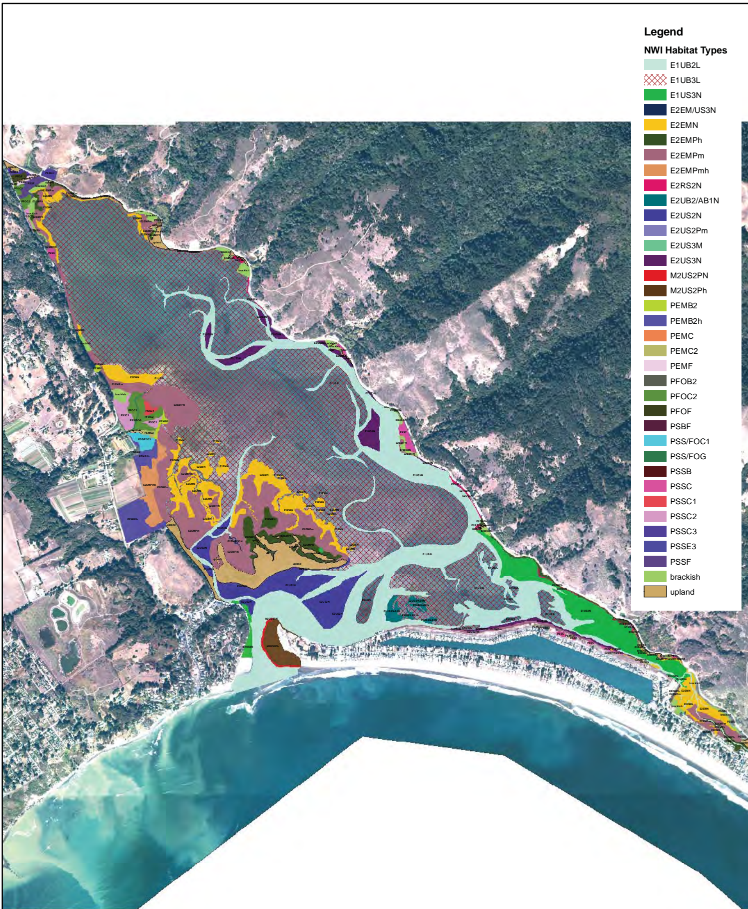
Figure A -12. Year 0 Map of NWI Wetland Habitat Types
