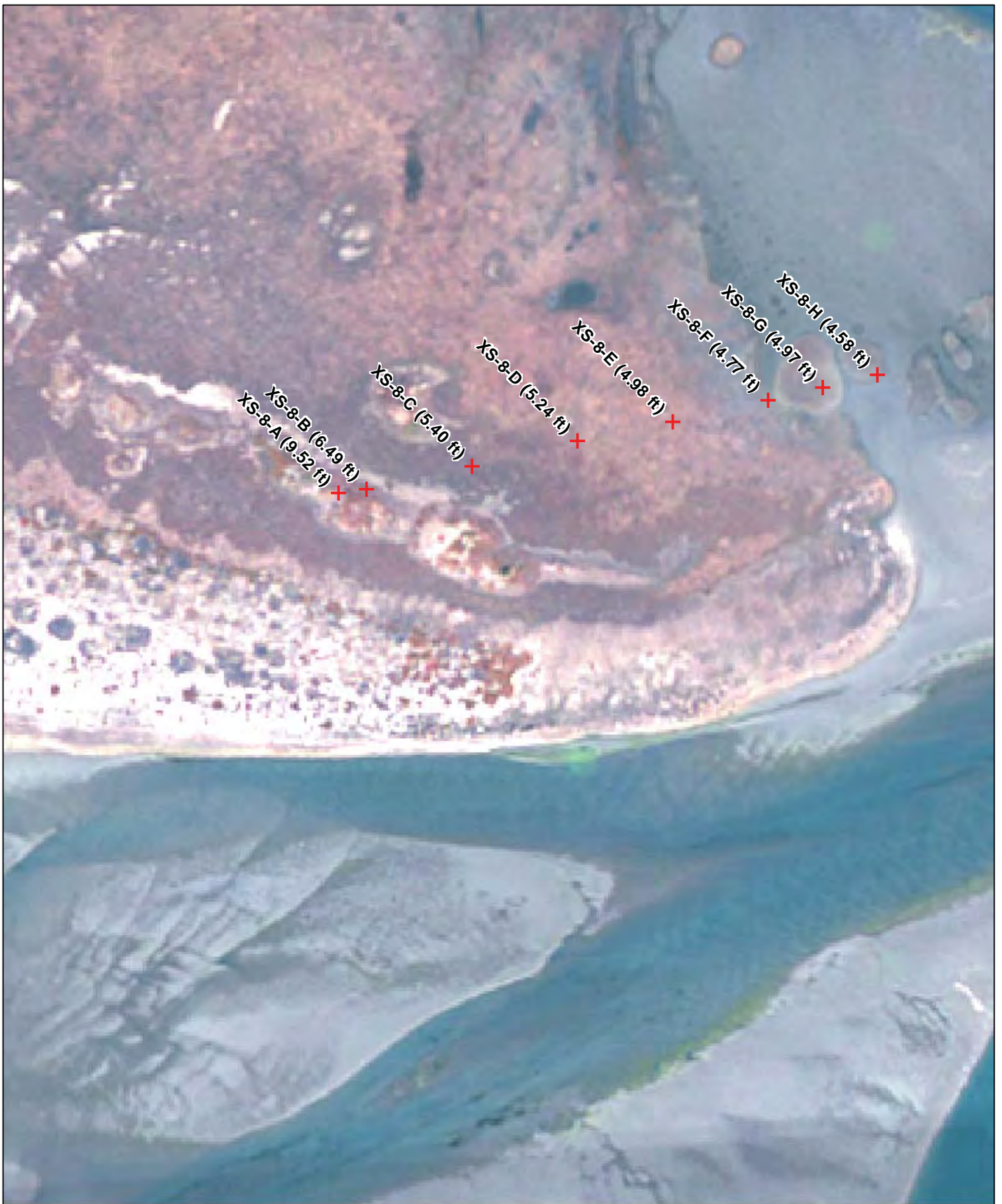
Figure A-5f. Layout of Transect on Kent Island
